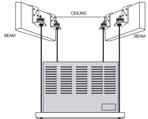
FURNACE INSTALLATION
