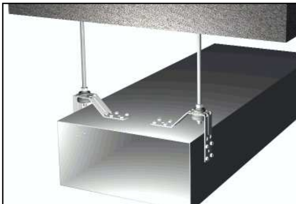
Square duct fastened to ceiling using fasteners, threaded rod and steel anchors.
